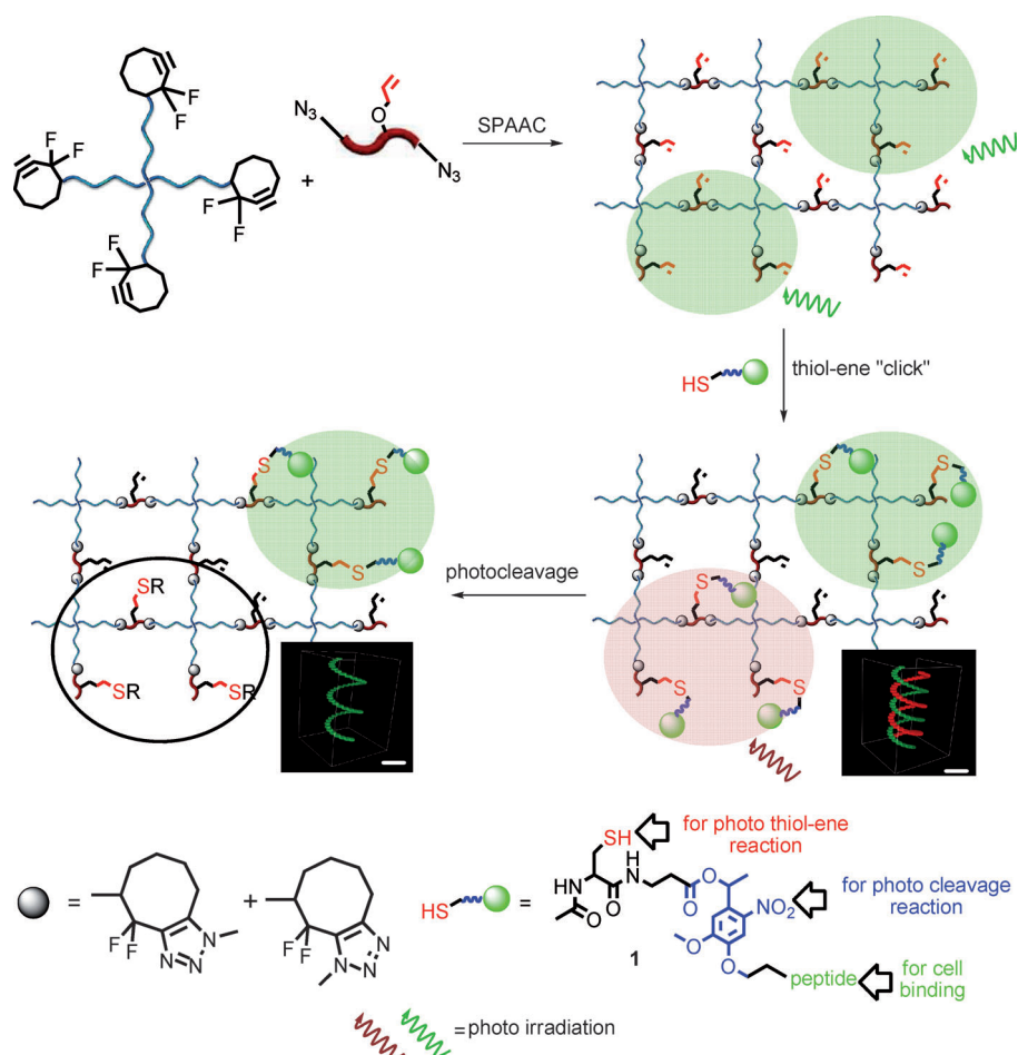
Figure 1. Illustration of the synthetic approach, which involves three bioorthogonal chemistries. The hydrogel network is formed by a SPAAC reaction between difluorocyclooctyne-terminated polyethylene glycol and bis-azido crosslinkers. These anchor points (as indicated by gray spheres and red highlighted line) also contain an overhanging alkenyl group for photoinduced thiol-ene chemistry to regioselectively confine the bioactive ligands. The ligand 1 contains a reactive thiol group (red) for thiol-ene chemistry, and a biorelevant, fluorescent peptide group (green) bridged by a photocleavable o -nitrophenyl ether (blue). To demonstrate the chemical selectivity and spatial resolution, two different, fluorescently labeled ligands (red and green) are positioned in a helical arrangement by thiol-ene “click” (bottom right inset). The ligands with the red fluorophore peptide conjugates are then selectively removed by cleavage of the o -nitrobenzyl group, which leaves only the ligands with the green fluorophore (bottom left inset).
